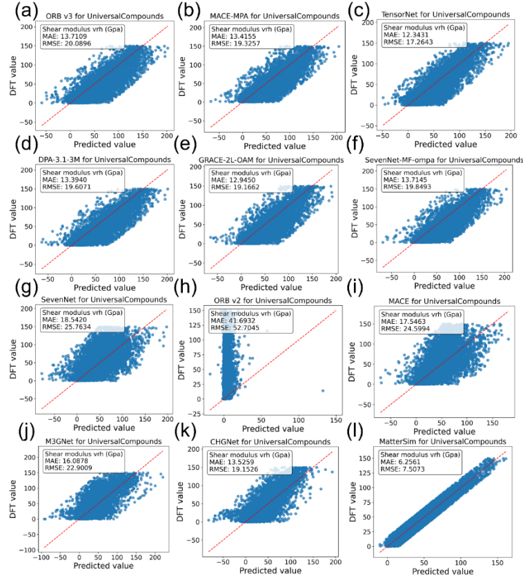
Figure S4 evaluates the performance of 12 MLIPs on the MP shear modulus universal test dataset, comparing their predictions with DFT results.
