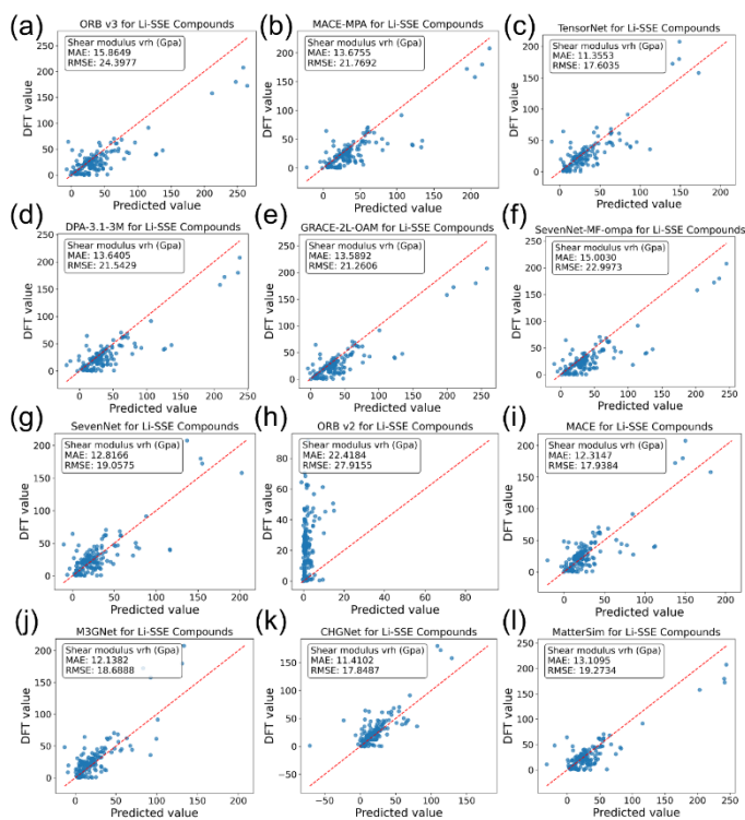
Figure S6 presents the performance of 12 MLIPs on the MP shear modulus lithium solid electrolyte test dataset, comparing their predictions with DFT results.
