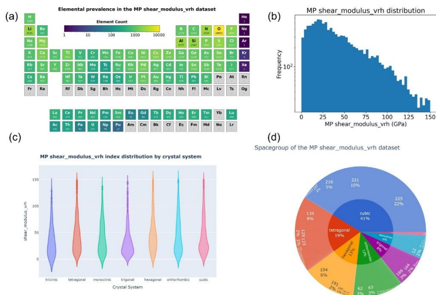
Figure S1 presents the visualization analysis results of 10,812 shear modulus structures selected from the MP database as a general test dataset. These structures were extracted from 12,334 raw structures and include: (a) Visualization of element distribution; (b) Histogram of shear modulus values; (c) Distribution of shear modulus values based on crystal system classification; (d) Pie chart of shear modulus dataset classified by crystal system and corresponding space groups.
