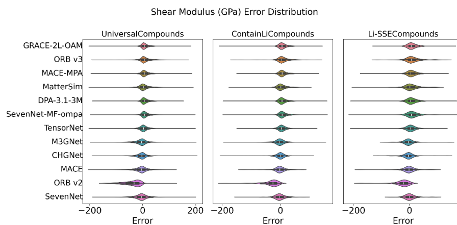
Figure S7 presents error distribution plots comparing the predictions of 12 MLIPs with DFT results on the UniversalCompounds, ContainLiCompounds, and Li-SSECompounds datasets (three levels of the MP shear modulus test set).
