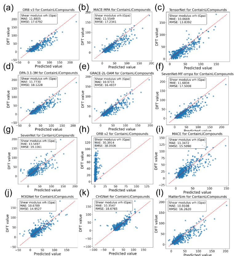
Figure S5 evaluates the performance of 12 MLIPs on the MP shear modulus lithium compound test dataset, comparing their predictions with DFT results. .
