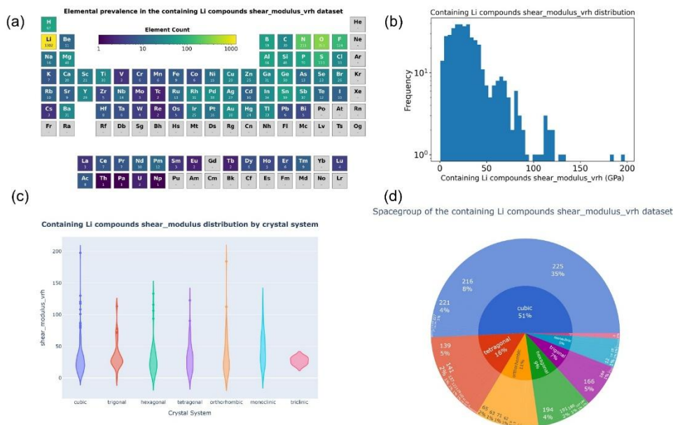
Figure S2 presents the visualization analysis results of 422 structures extracted from the remaining lithium-containing structures in the MP shear modulus dataset after excluding the general test dataset, serving as a lithium compound test dataset. The contents include: (a) Visualization of element distribution; (b) Histogram of shear modulus values; (c) Distribution of shear modulus values based on crystal system classification; (d) Pie chart of shear modulus dataset classified by crystal system and corresponding space groups.
