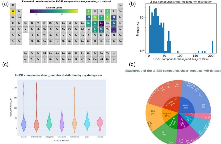
Figure S3 presents the visualization analysis results of 153 structures extracted from the remaining lithium-containing structures in the MP shear modulus dataset after excluding the general test dataset, serving as a lithium solid electrolyte test dataset. The contents include: (a) Visualization of element distribution; (b) Histogram of shear modulus values; (c) Distribution of shear modulus values based on crystal system classification; (d) Pie chart of shear modulus dataset classified by crystal system and corresponding space groups.
